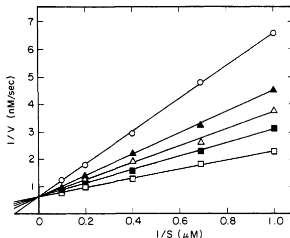
Figure 1. Inhibition of chorismate synthase by iso-EPSP, 3. Assays were conducted at 29.6 °C, pH 7.8 (Tris-HCl), and included in a final volume of 2.0 mL 3.14 \mu\text{kat} of chorismate synthase, 440 \mu\text{kat} of anthranilate synthase, 10 \mu\text{M} FMN, 44 \mu\text{M} NADPH, 5 mM glutamine, 50 mM Tris buffer, 50 mM KCl, and 2.5 mM \text{MgCl}_2 , in addition to substrate EPSP (1) and iso-EPSP (3); reaction velocity was monitored by the increase in fluorescence (excitation at 313 nm, emission at 390 nm). 12 Inhibitor concentrations: (□) no inhibitor, (■) 1 \mu\text{M} , (△) 2.5 \mu\text{M} , (▲) 5 \mu\text{M} , and (○) 10 \mu\text{M} .
